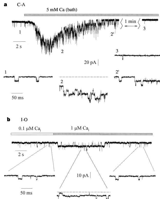
Figure 3 Activity of PCL single channels is increased by \text{Ca}^{2+} . a , Top, single-channel currents recorded at -60 mV in a cell-attached patch before and after adding 5 mM \text{Ca}^{2+} to the bath ( \text{Na}_o solution). The pipette solution was K140. Bottom, expanded traces representing, respectively, the resting (1), activated (2, 2') and desensitized (3) states. Resting potential of oocytes was assumed to be -30 mV. b , Representative traces at -50 mV in an inside-out patch before and after adding 1 \mu\text{M} \text{Ca}_i^{2+} (top). Selected traces are expanded (bottom). Open probabilities were 0.14 \pm 0.03 , 0.58 \pm 0.12 , and 0.10 \pm 0.02 ( n = 8 ), for the resting, activated and desensitized states, respectively. The pipette solution was \text{Na}_o and the intracellular solution was \text{K}_o supplemented with 5 \text{CaK}_2\text{EGTA} + \text{H}_2\text{K}_2\text{EGTA} to obtain 0.1 or 1 \mu\text{M} free \text{Ca}^{2+} .
